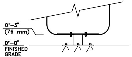
2811-DT-P (PEDESTAL MOUNT) SCALE: 3/4"=1'-0"
