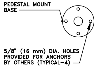
2811-DT-E (EMBEDMENT) SCALE: 3/4"=1'-0"
